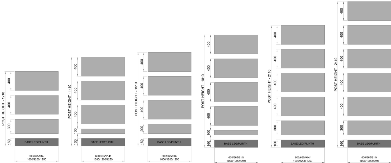
Backpanel Diagram - Plain & Volcano Correct backpanel layout for each upright height.
